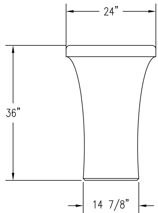
2 ELEVATION VIEW
