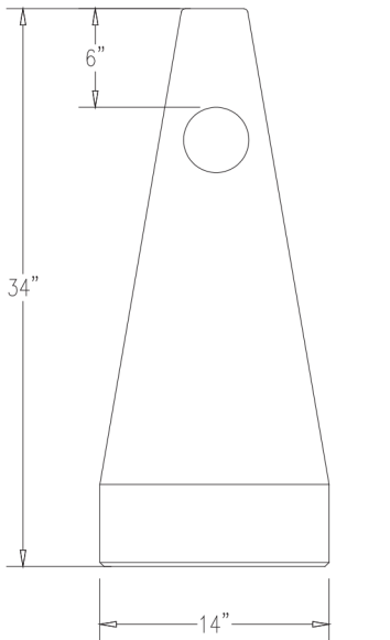
ELEVATION VIEW
