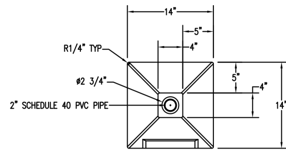
1 TOP VIEW OF SNUFFER
