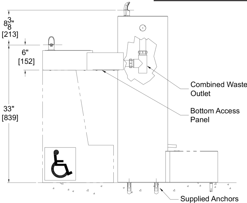
OPTIONAL -PF PET FOUNTAIN DETAIL
