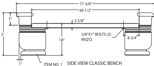
SIDE VIEW CLASSIC BENCH
