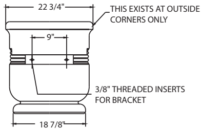
BENCH END INSIDE END VIEW
