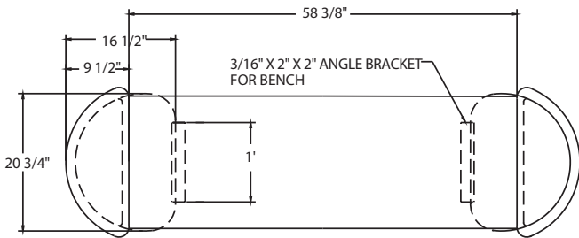
TOP VIEW CLASSIC BENCH
