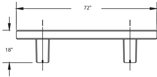
SIDE ELEVATION CAST CONCRETE BENCH
