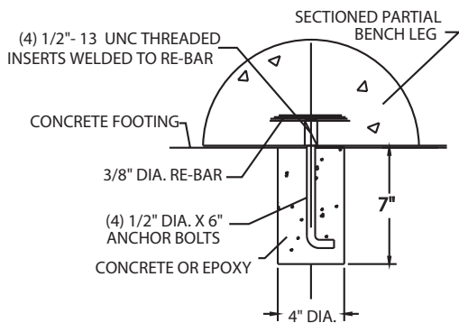
SECTIONED ANCHORING SYSTEM DETAIL
