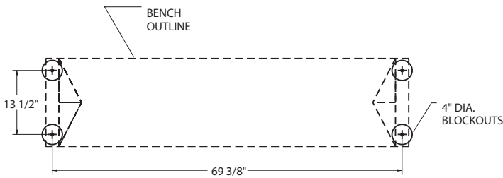
BLOCKOUT POSITIONS FOR ANCHORING
