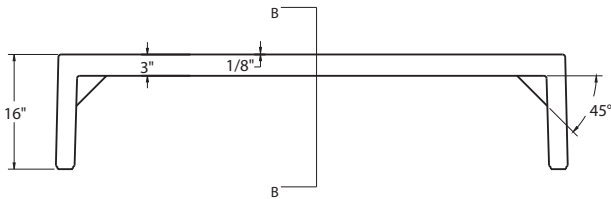
FRONT VIEW LAKESIDE BENCH
